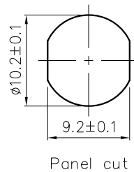
Panel cut
